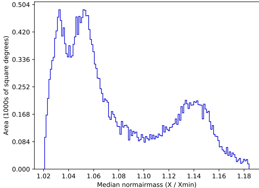
ddf_acor_sf20_lsf40_lsr10_v3.4_10yrs All sky all bands: Median normairmass
