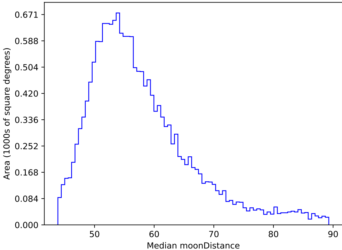
ddf_acor_sf20_lsf40_lsr10_v3.4_10yrs WFD y band: Median moonDistance
