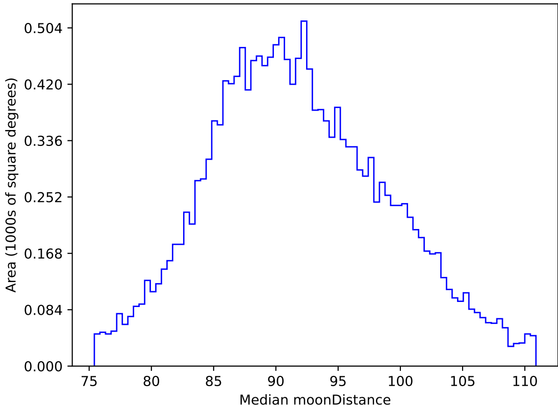
ddf_acor_sf20_lsf40_lsr10_v3.4_10yrs WFD i band: Median moonDistance
