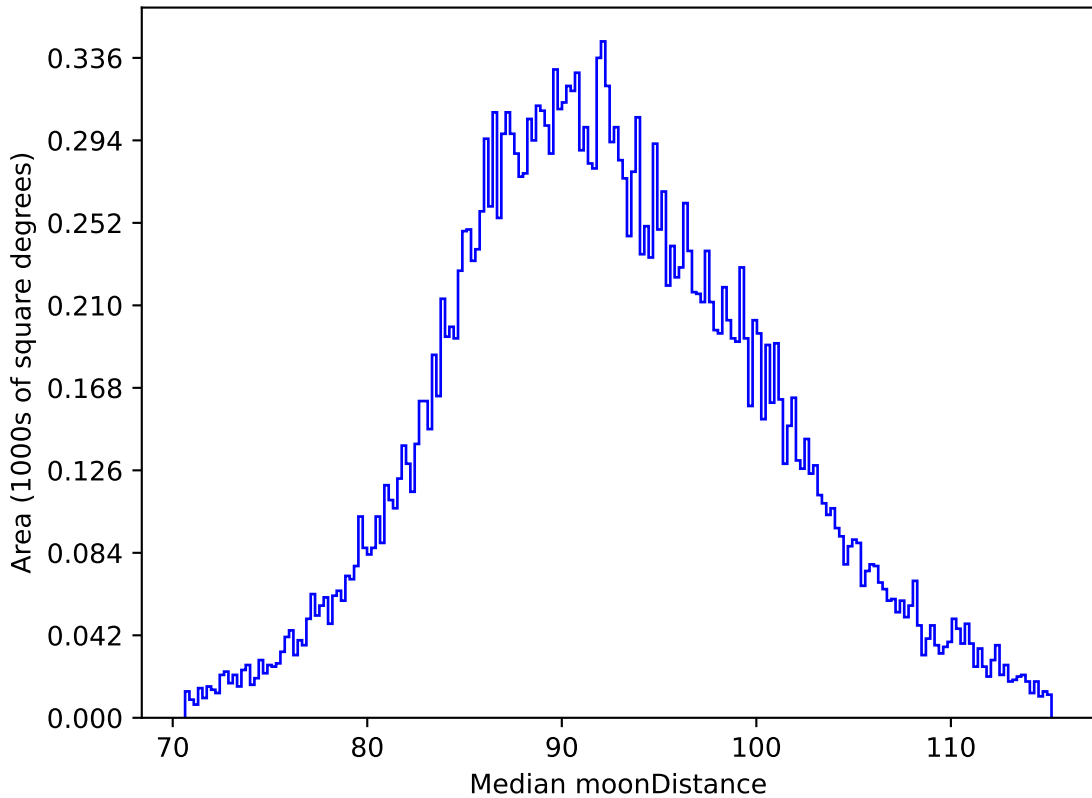
ddf_acor_sf20_lsf40_lsr10_v3.4_10yrs All sky i band: Median moonDistance
