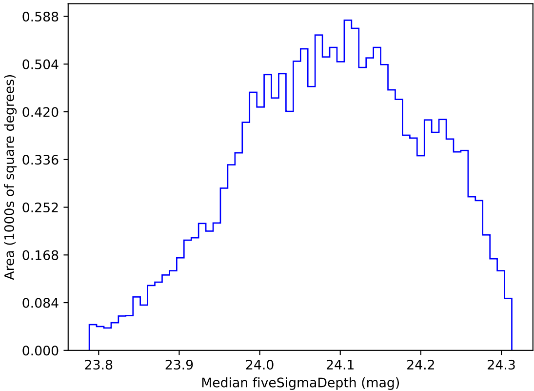
ddf_acor_sf20_lsf40_lsr10_v3.4_10yrs WFD r band: Median fiveSigmaDepth
