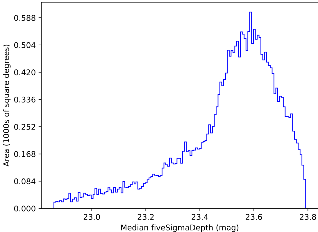
ddf_acor_sf20_lsf40_lsr10_v3.4_10yrs All sky i band: Median fiveSigmaDepth
