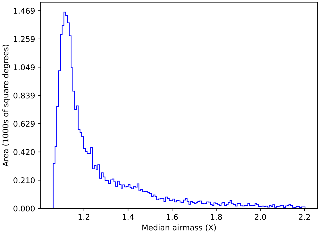
ddf_acor_sf20_lsf40_lsr10_v3.4_10yrs Yr 1 z band: Median airmass
