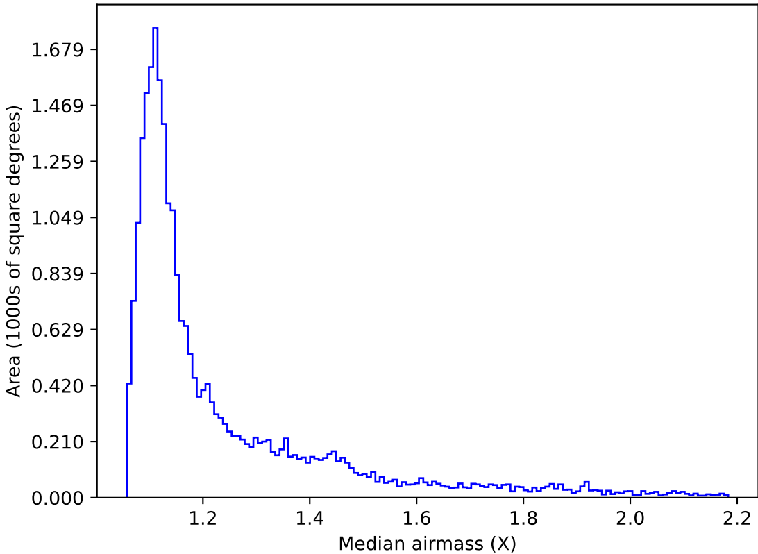
ddf_acor_sf20_lsf40_lsr10_v3.4_10yrs Yr 1 i band: Median airmass
