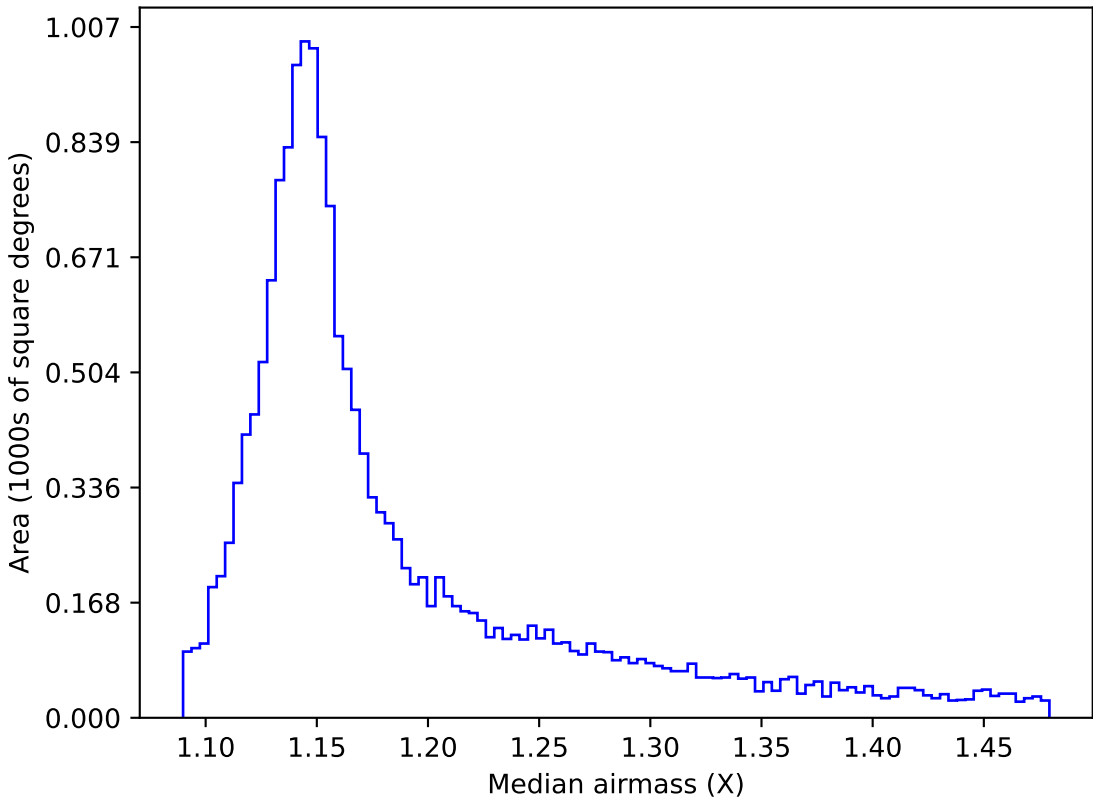
ddf_acor_sf20_lsf40_lsr10_v3.4_10yrs WFD y band: Median airmass
