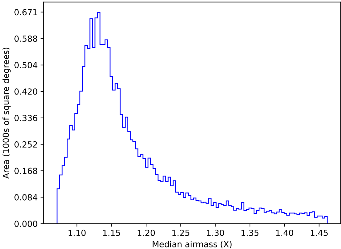
ddf_acor_sf20_lsf40_lsr10_v3.4_10yrs WFD u band: Median airmass
