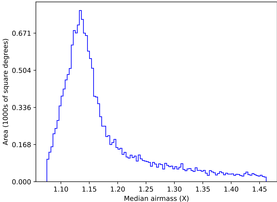
ddf_acor_sf20_lsf40_lsr10_v3.4_10yrs WFD r band: Median airmass
