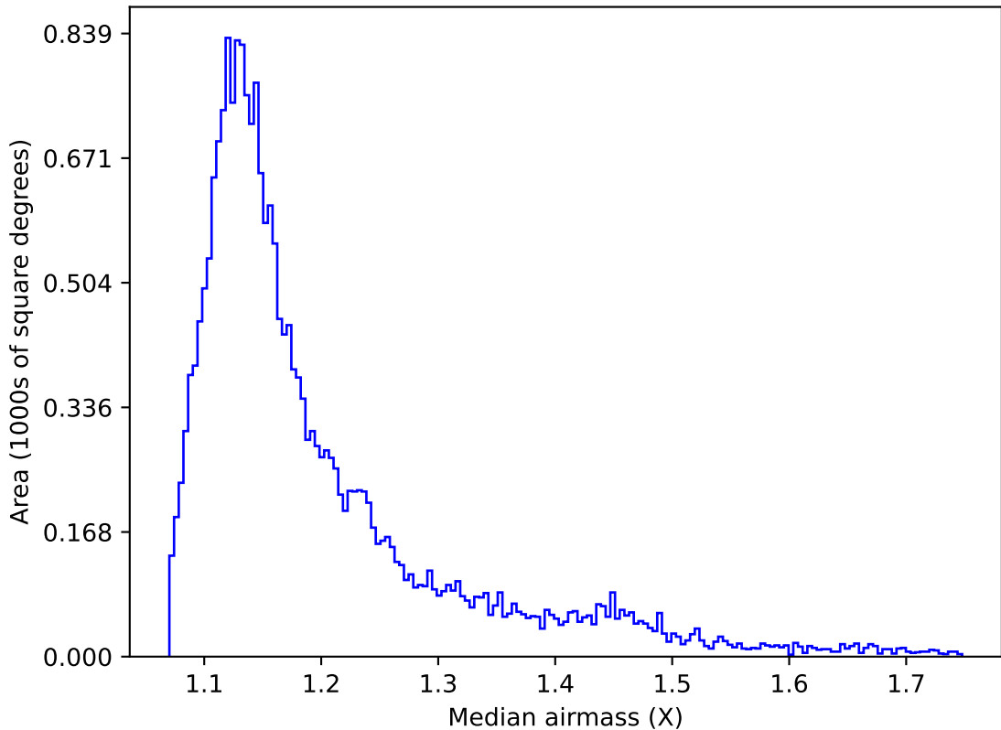
ddf_acor_sf20_lsf40_lsr10_v3.4_10yrs All sky u band: Median airmass
