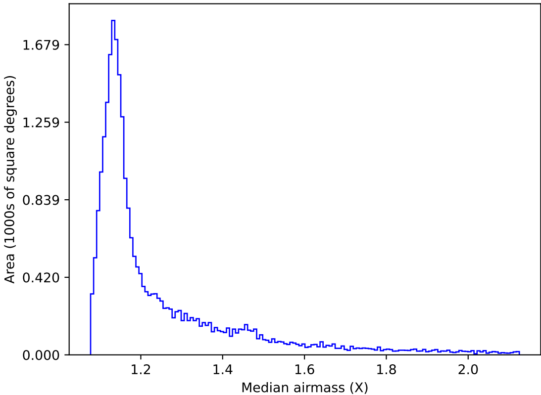
ddf_acor_sf20_lsf40_lsr10_v3.4_10yrs All sky r band: Median airmass
