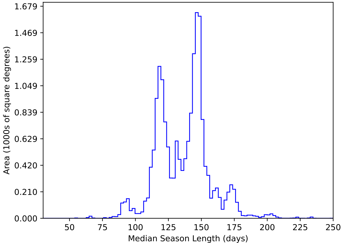
ddf_acor_sf20_lsf40_lsr10_v3.4_10yrs WFD y band: Median Season Length
