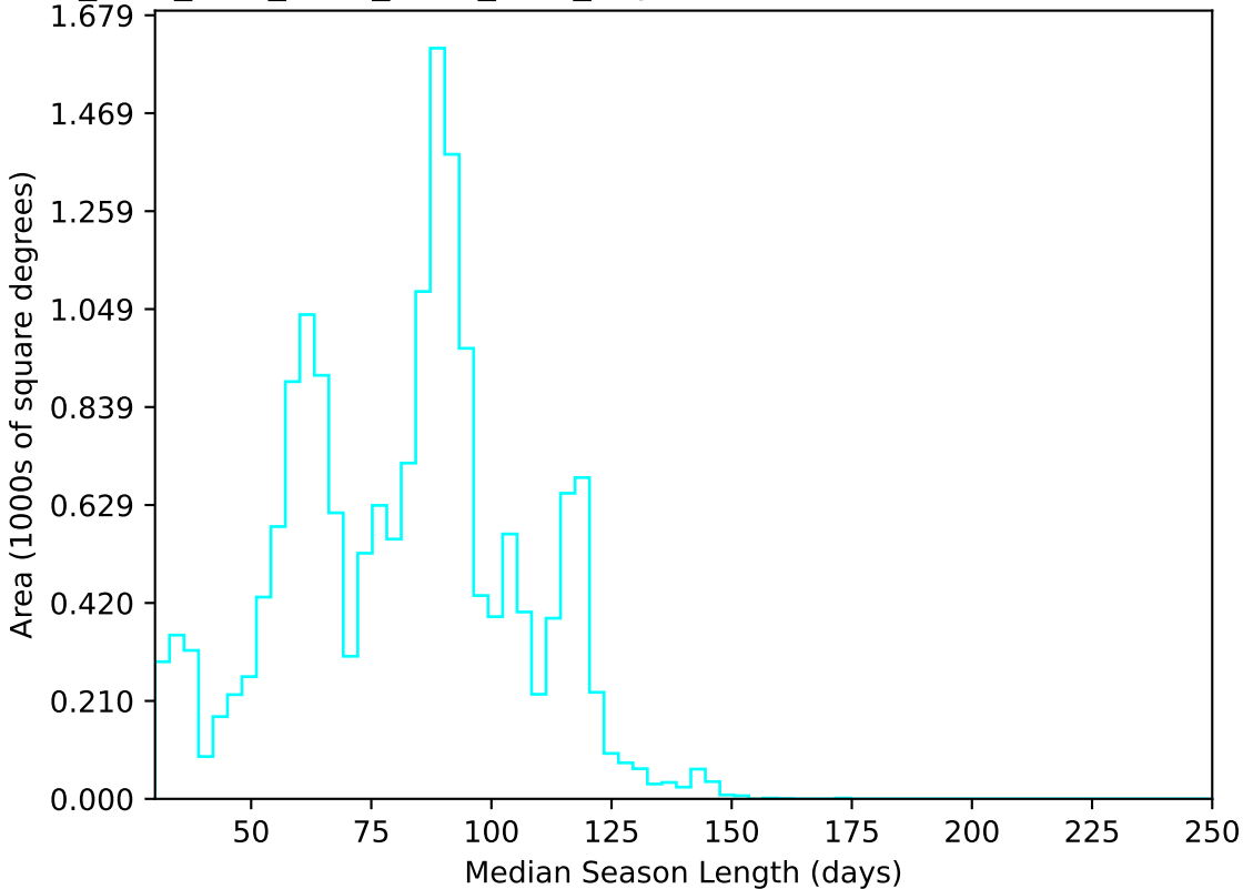
ddf_acor_sf20_lsf40_lsr10_v3.4_10yrs WFD u band: Median Season Length
