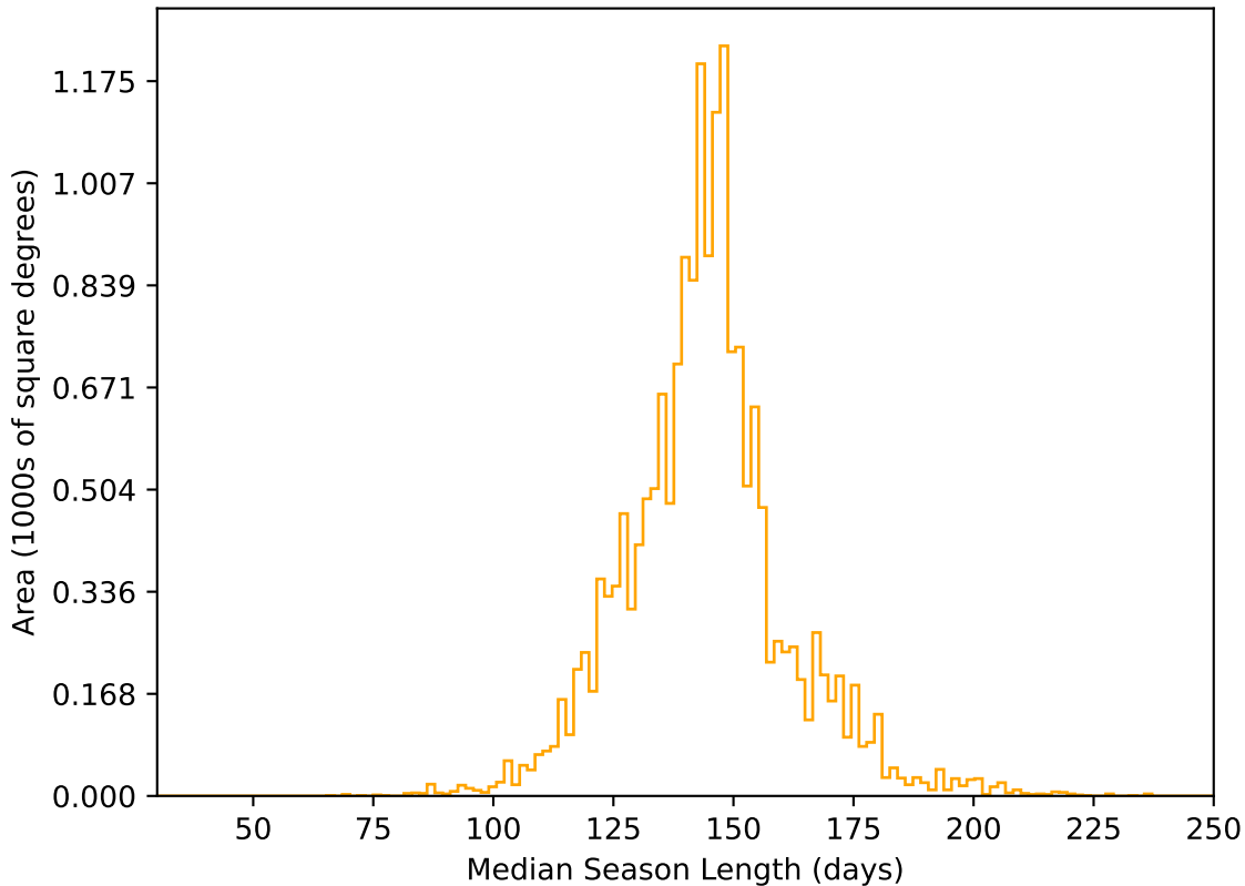
ddf_acor_sf20_lsf40_lsr10_v3.4_10yrs WFD r band: Median Season Length
