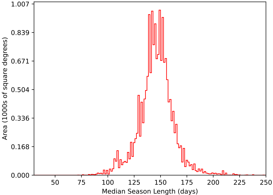
ddf_acor_sf20_lsf40_lsr10_v3.4_10yrs WFD i band: Median Season Length
