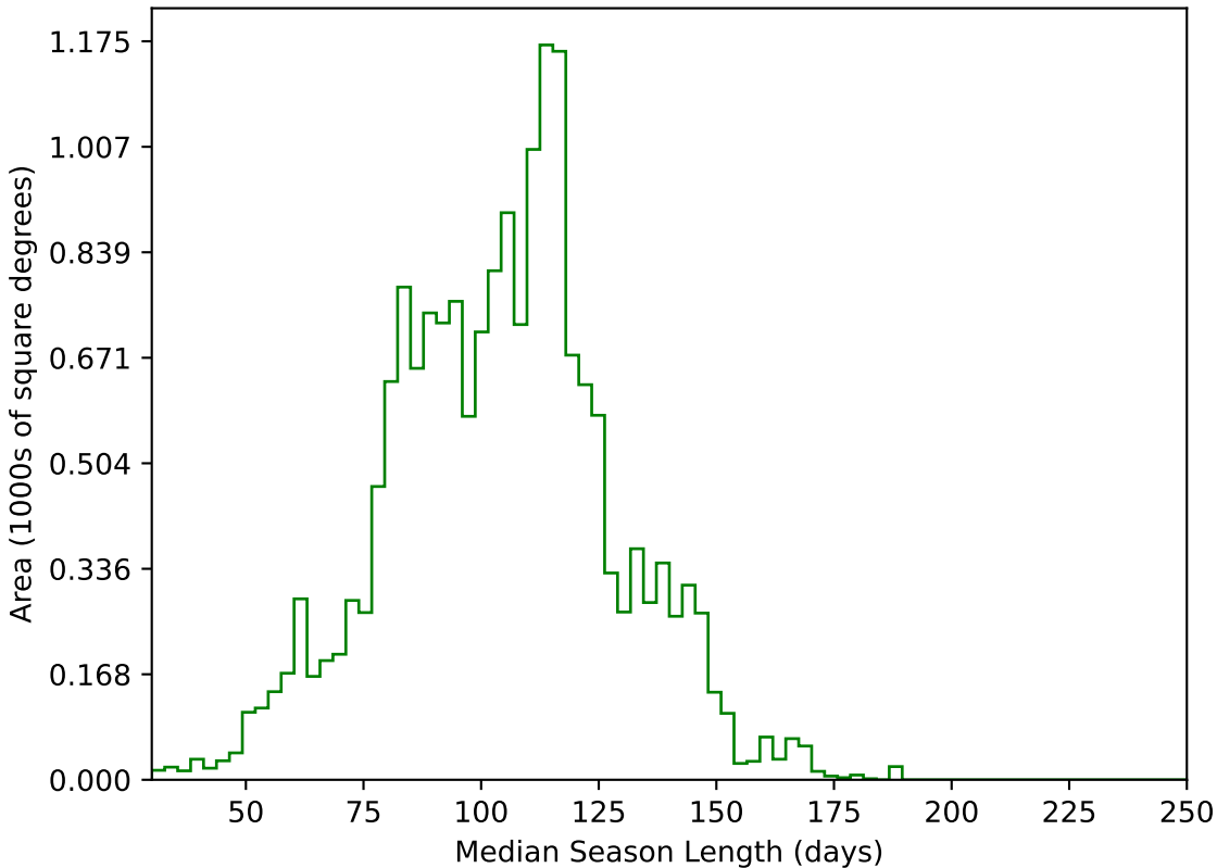
ddf_acor_sf20_lsf40_lsr10_v3.4_10yrs WFD g band: Median Season Length
