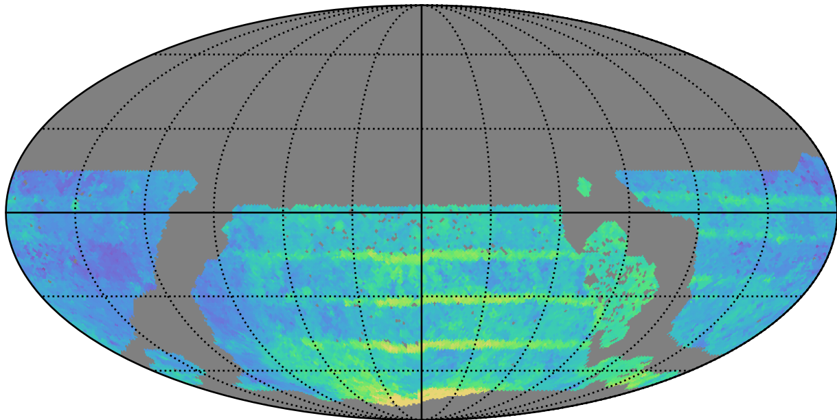
ddf_acor_sf20_lsf40_lsr10_v3.4_10yrs WFD all bands: Median Season Length
