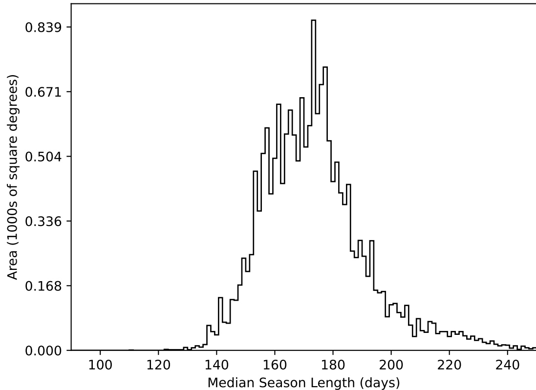
ddf_acor_sf20_lsf40_lsr10_v3.4_10yrs WFD all bands: Median Season Length
