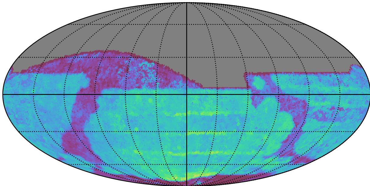
ddf_acor_sf20_lsf40_lsr10_v3.4_10yrs All sky z band: Median Season Length
