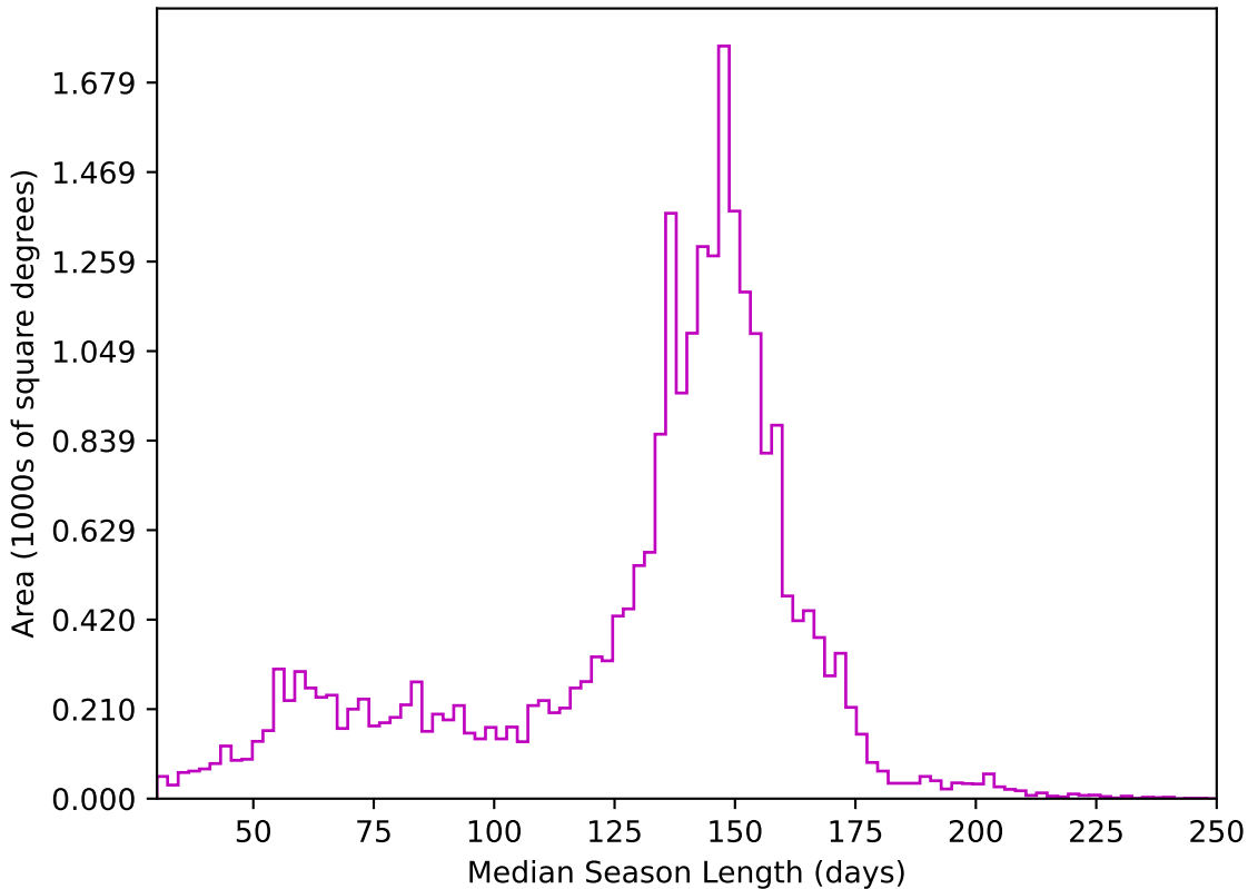
ddf_acor_sf20_lsf40_lsr10_v3.4_10yrs All sky z band: Median Season Length
