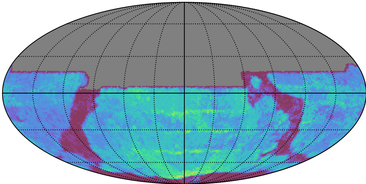
ddf_acor_sf20_lsf40_lsr10_v3.4_10yrs All sky y band: Median Season Length
