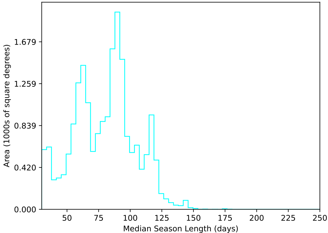
ddf_acor_sf20_lsf40_lsr10_v3.4_10yrs All sky u band: Median Season Length
