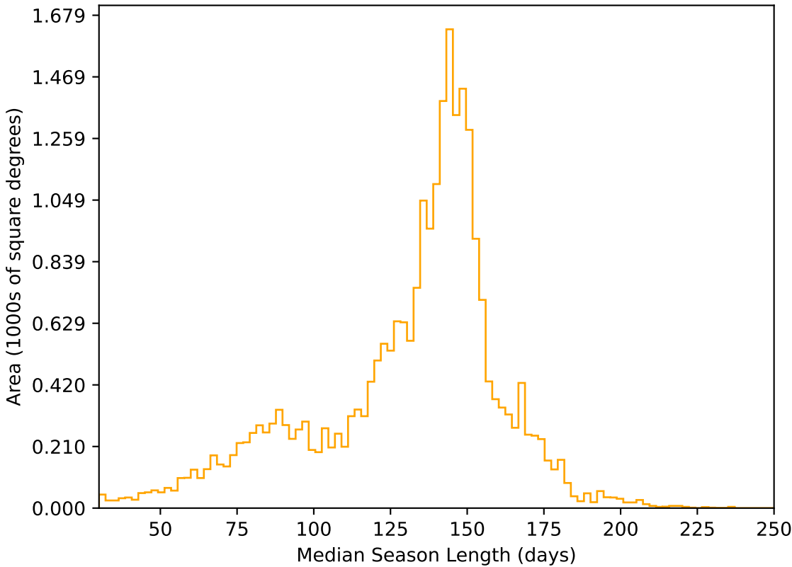
ddf_acor_sf20_lsf40_lsr10_v3.4_10yrs All sky r band: Median Season Length
