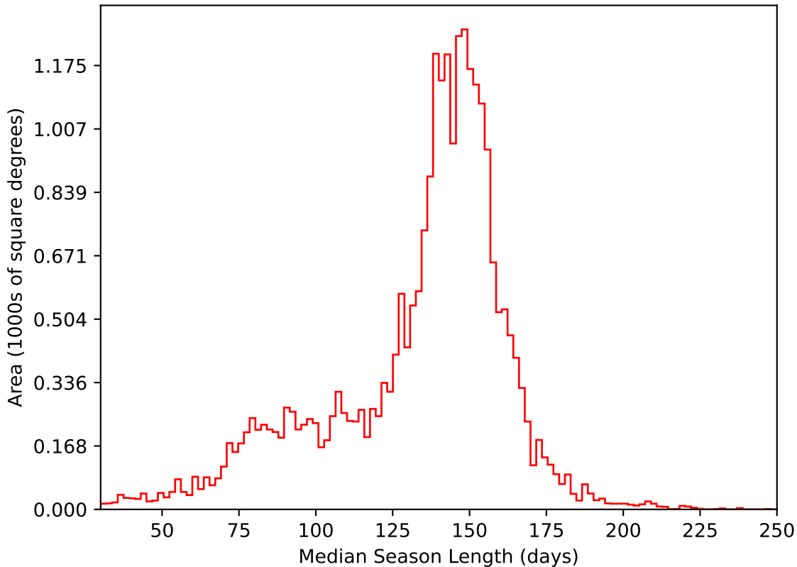
ddf_acor_sf20_lsf40_lsr10_v3.4_10yrs All sky i band: Median Season Length
