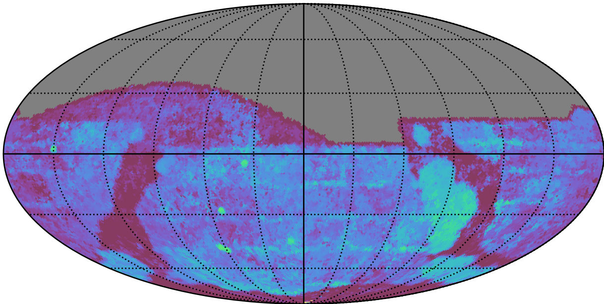
ddf_acor_sf20_lsf40_lsr10_v3.4_10yrs All sky g band: Median Season Length
