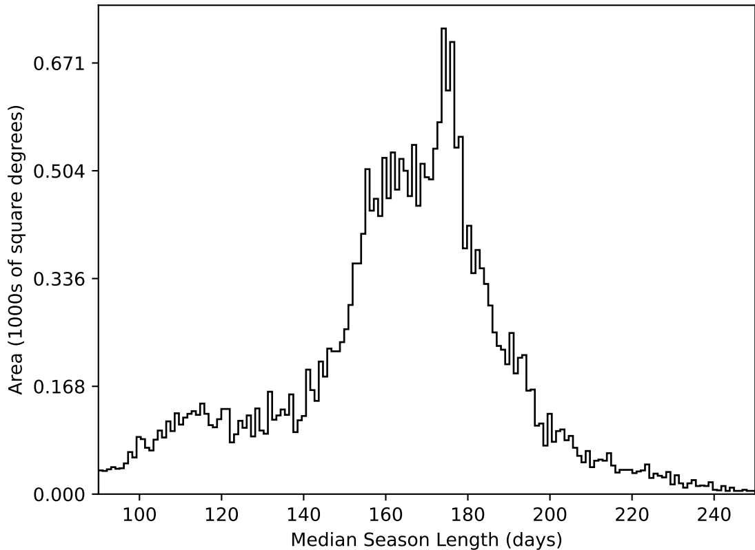
ddf_acor_sf20_lsf40_lsr10_v3.4_10yrs All sky all bands: Median Season Length
