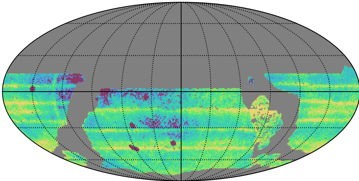
ddf_acor_sf20_lsf40_lsr10_v3.4_10yrs WFD: Median Intra-Night Gap
