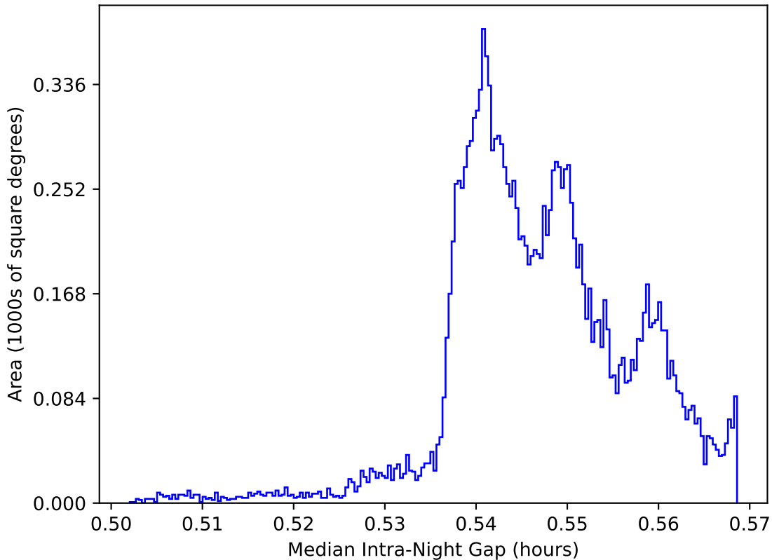
ddf_acor_sf20_lsf40_lsr10_v3.4_10yrs WFD: Median Intra-Night Gap
