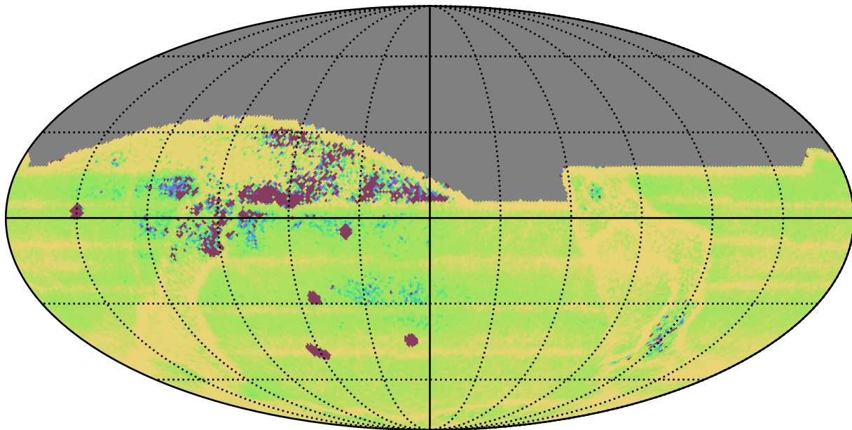
ddf_acor_sf20_lsf40_lsr10_v3.4_10yrs All sky: Median Intra-Night Gap
