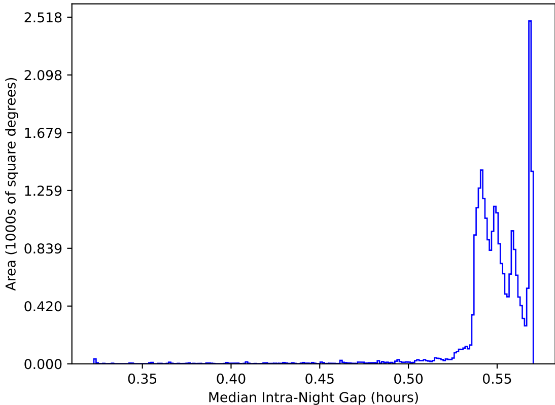
ddf_acor_sf20_lsf40_lsr10_v3.4_10yrs All sky: Median Intra-Night Gap
