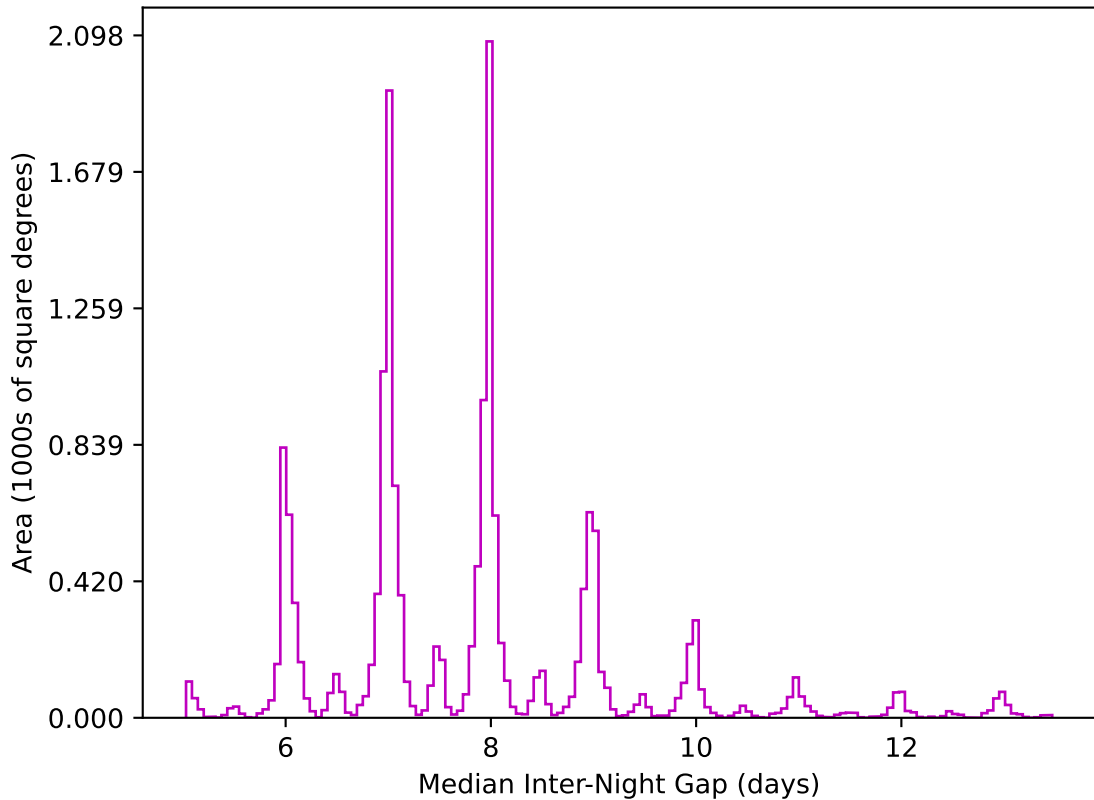
ddf_acor_sf20_lsf40_lsr10_v3.4_10yrs WFD z band: Median Inter-Night Gap
