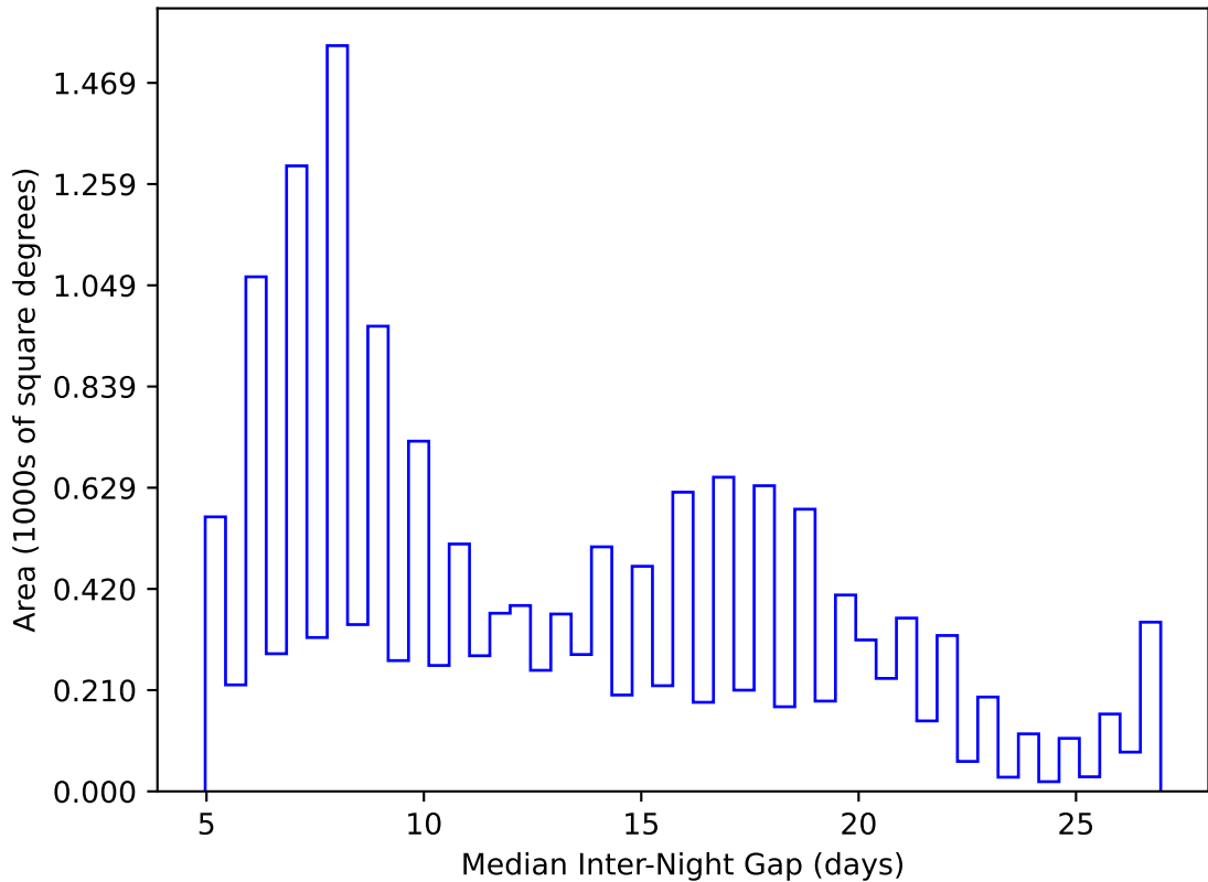
ddf_acor_sf20_lsf40_lsr10_v3.4_10yrs WFD y band: Median Inter-Night Gap
