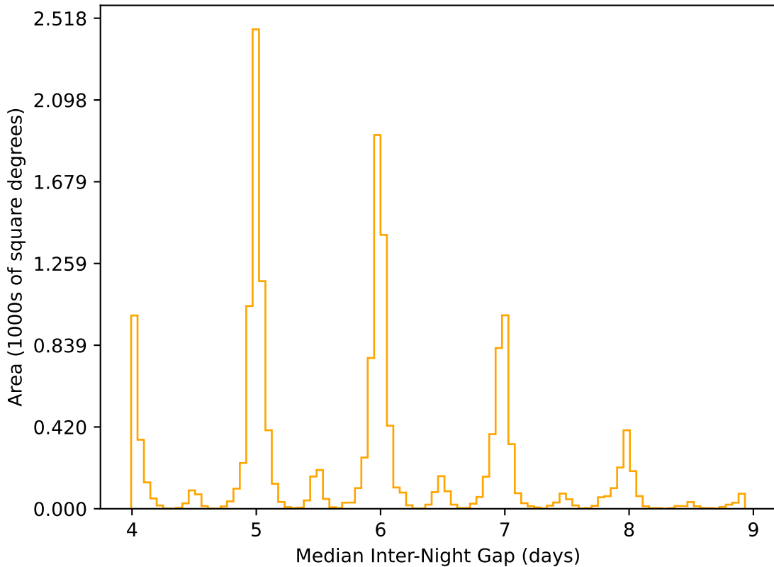
ddf_acor_sf20_ls40_lsr10_v3.4_10yrs WFD r band: Median Inter-Night Gap
