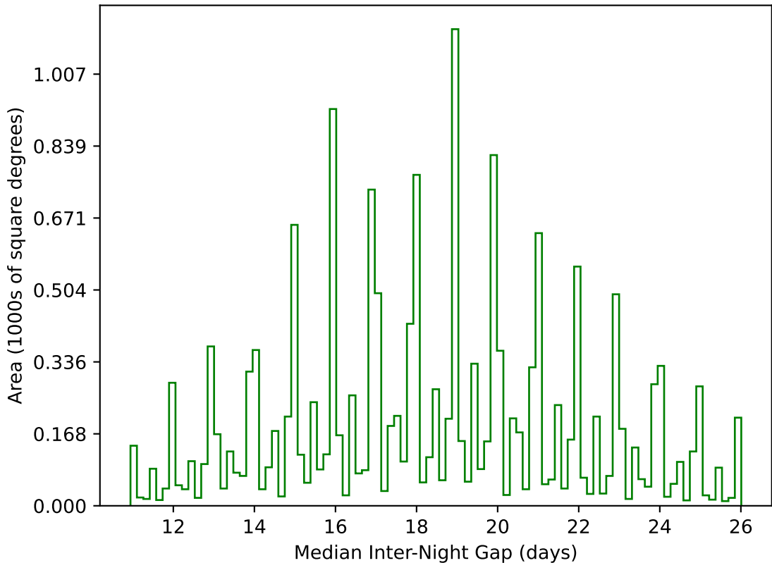
ddf_acor_sf20_lsf40_lsr10_v3.4_10yrs WFD g band: Median Inter-Night Gap
