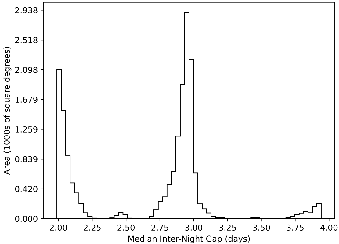
ddf_acor_sf20_lsf40_lsr10_v3.4_10yrs WFD all bands: Median Inter-Night Gap
