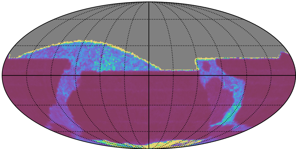
ddf_acor_sf20_lsf40_lsr10_v3.4_10yrs All sky z band: Median Inter-Night Gap
