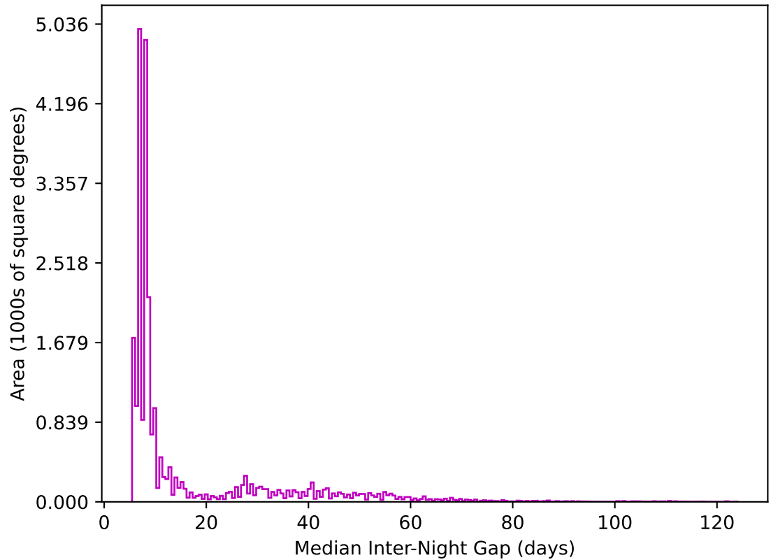
ddf_acor_sf20_lsf40_lsr10_v3.4_10yrs All sky z band: Median Inter-Night Gap
