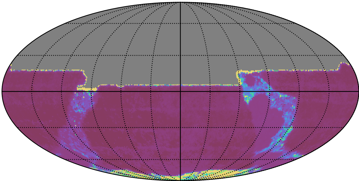
ddf_acor_sf20_lsf40_lsr10_v3.4_10yrs All sky y band: Median Inter-Night Gap
