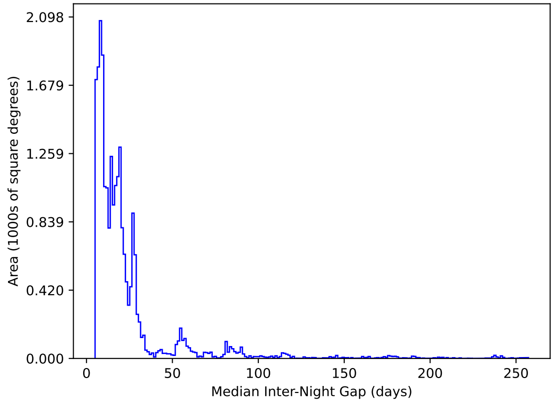
ddf_acor_sf20_lsf40_lsr10_v3.4_10yrs All sky y band: Median Inter-Night Gap
