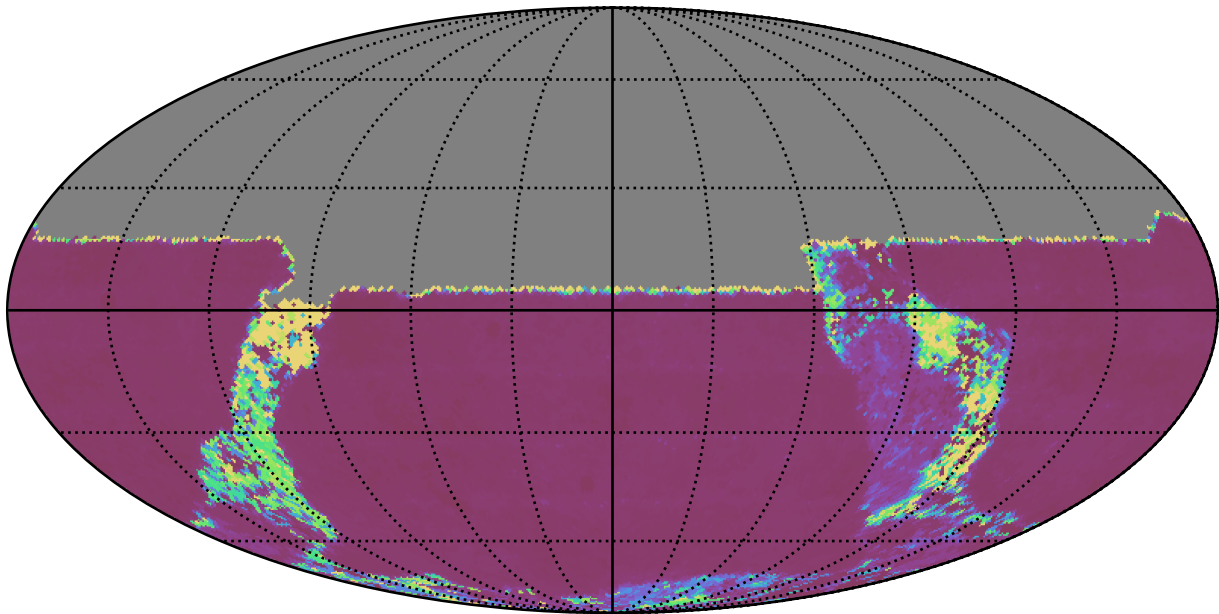
ddf_acor_sf20_lsf40_lsr10_v3.4_10yrs All sky u band: Median Inter-Night Gap
