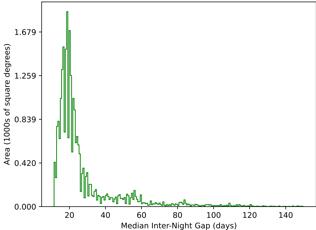
ddf_acor_sf20_lsf40_lsr10_v3.4_10yrs All sky g band: Median Inter-Night Gap
