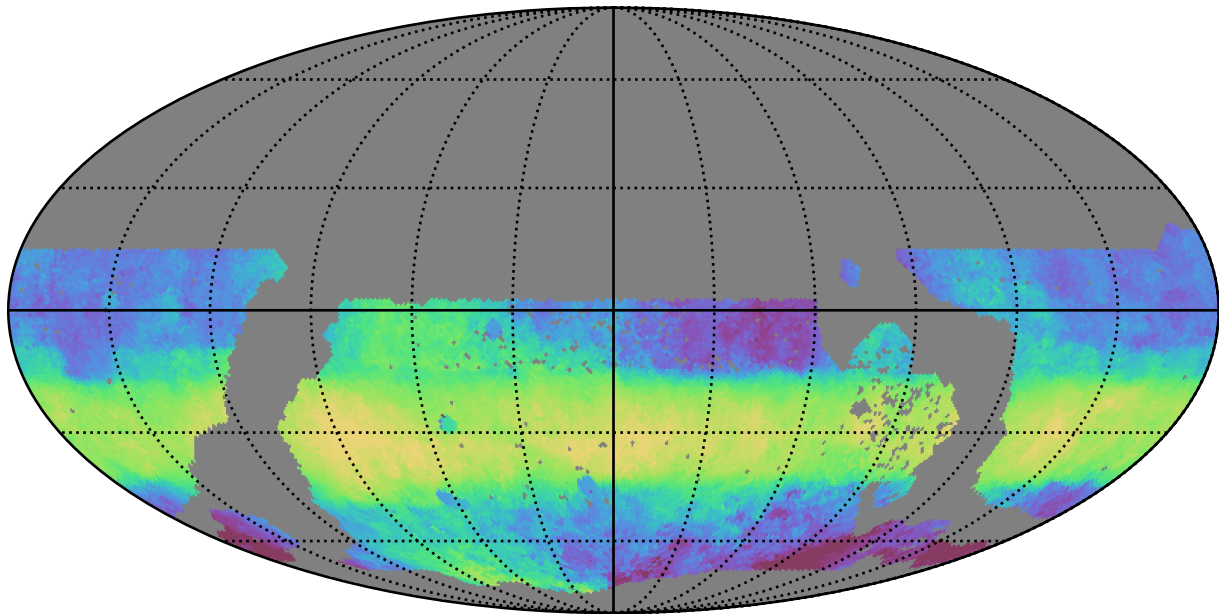
ddf_acor_sf20_lsf40_lsr10_v3.4_10yrs WFD z band: Median HA
