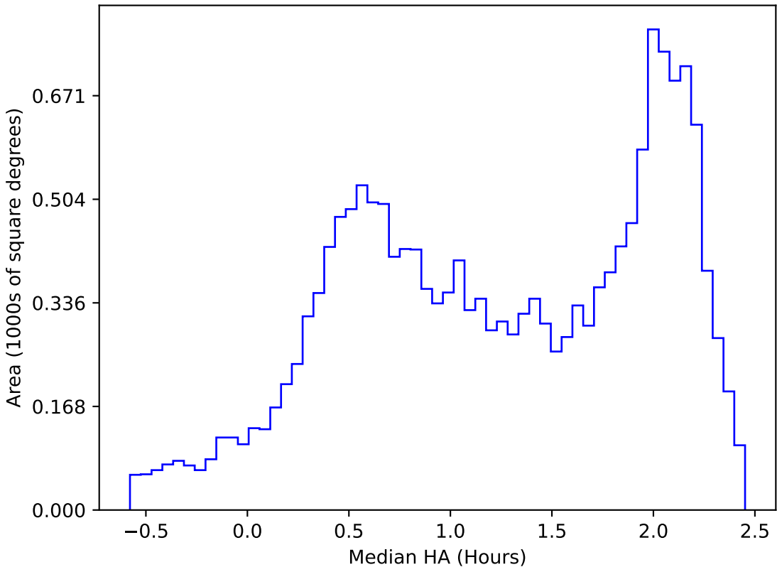
ddf_acor_sf20_lsf40_lsr10_v3.4_10yrs WFD y band: Median HA
