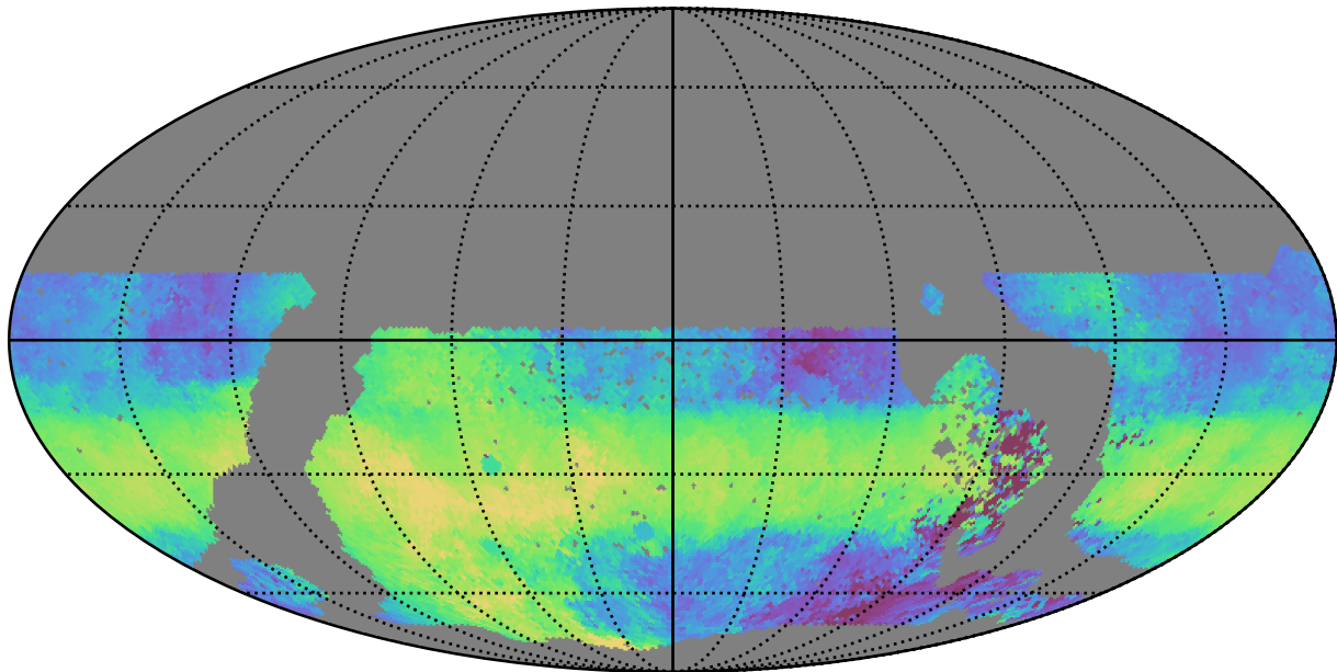
ddf_acor_sf20_lsf40_lsr10_v3.4_10yrs WFD u band: Median HA
