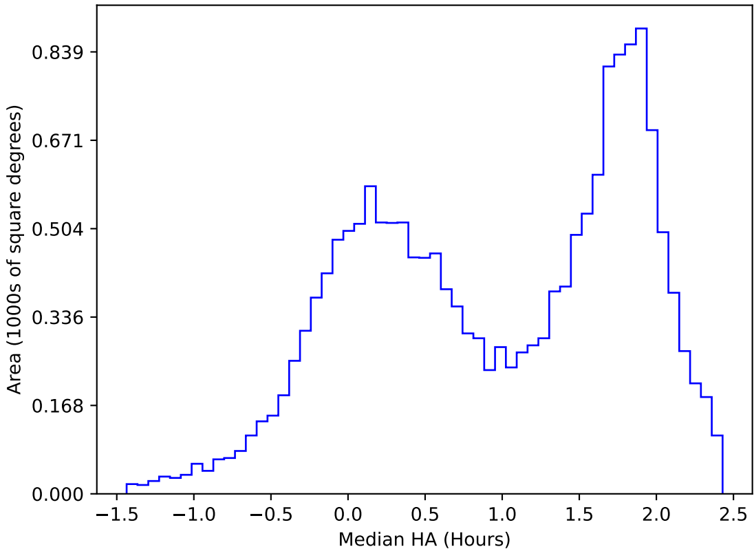
ddf_acor_sf20_lsf40_lsr10_v3.4_10yrs WFD u band: Median HA
