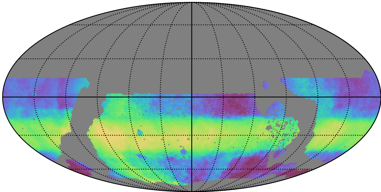
ddf_acor_sf20_lsf40_lsr10_v3.4_10yrs WFD r band: Median HA
