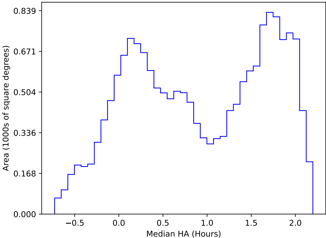
ddf_acor_sf20_lsf40_lsr10_v3.4_10yrs WFD r band: Median HA
