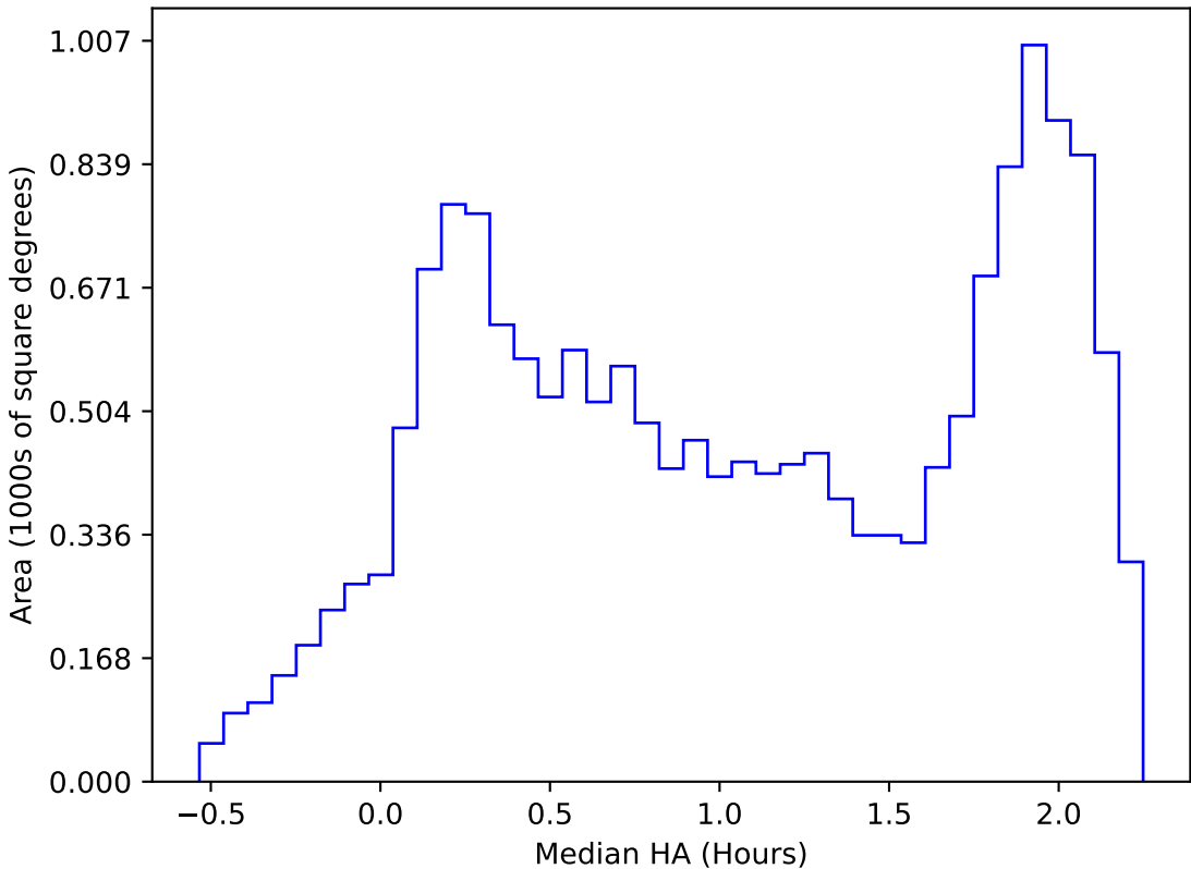
ddf_acor_sf20_lsf40_lsr10_v3.4_10yrs WFD i band: Median HA
